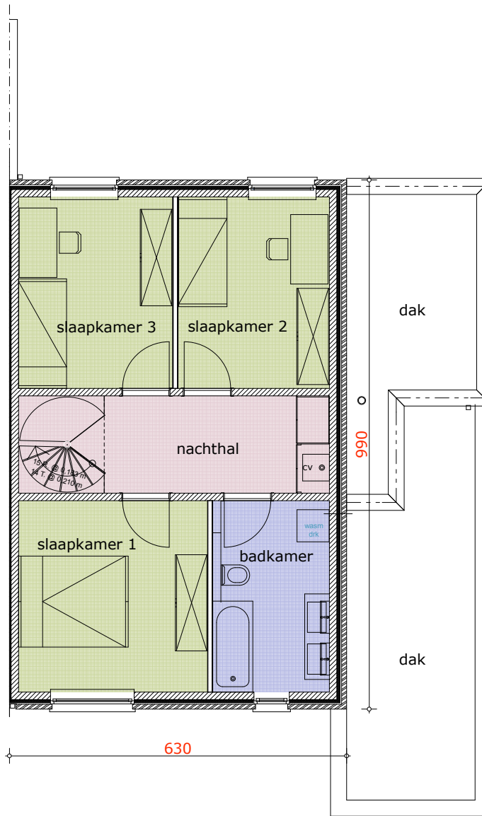
VERDIEPING woning 4-8
