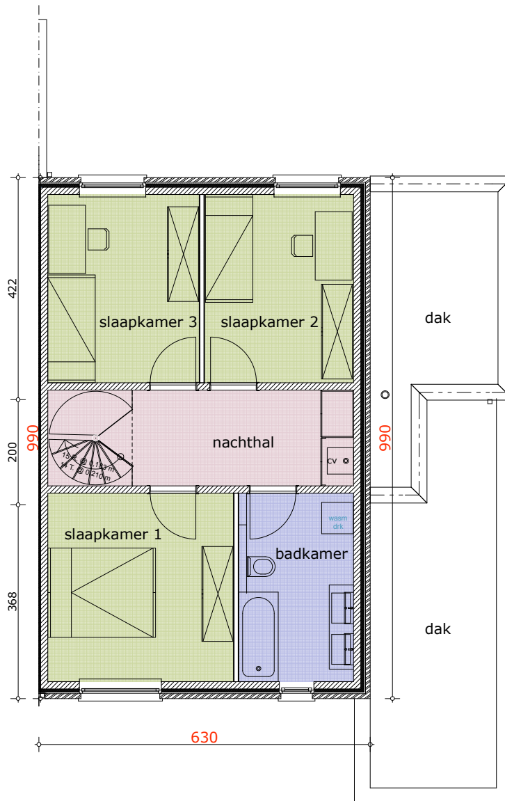
VERDIEPING woning 2-6
